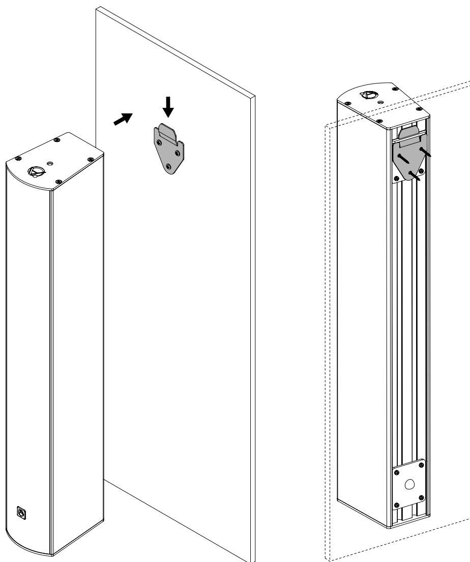
Figure 29: Hanging the loudspeaker module on the wall
