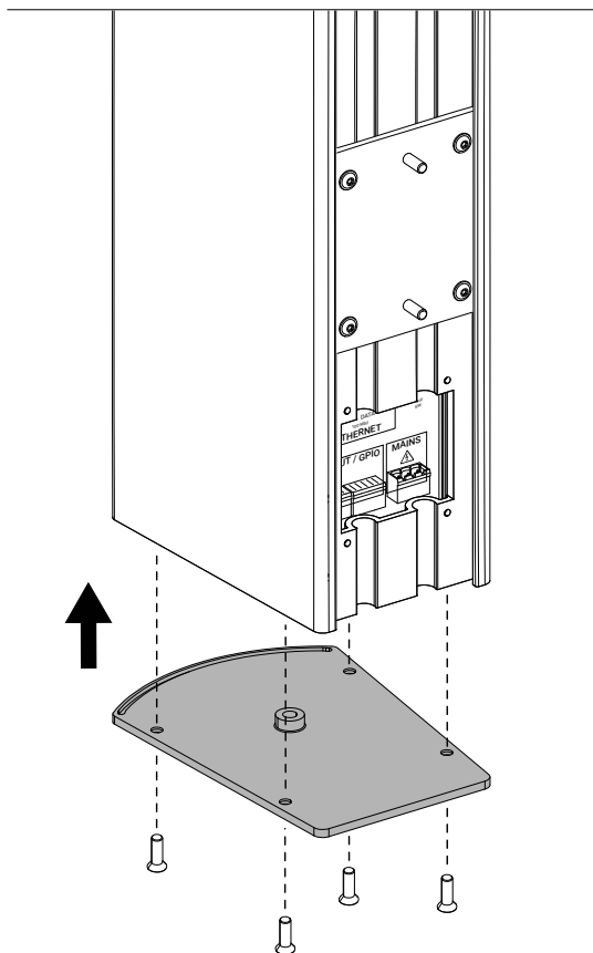
Figure 19: Replacing endcap
