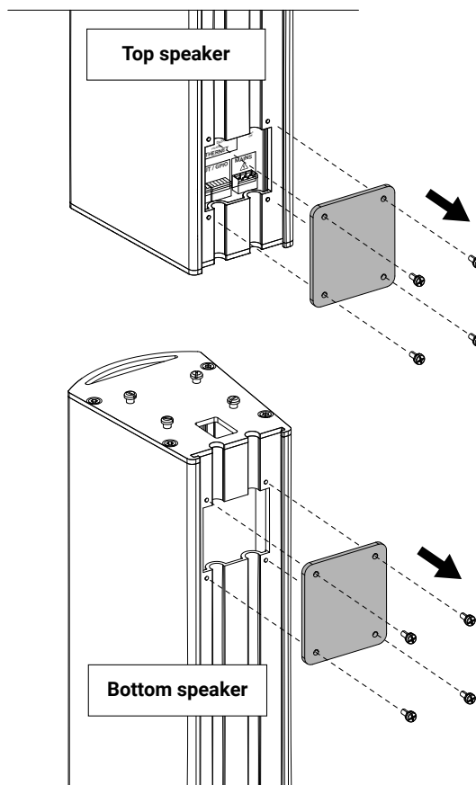
Figure 3: Removing connector plate covers
