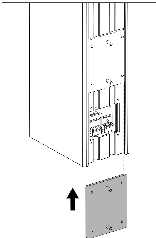
Figure 17: Sliding adaptor plate into grooves
