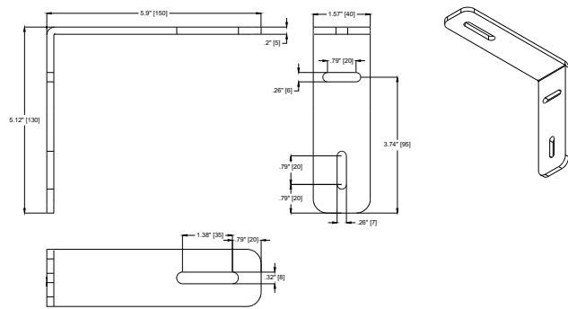
ALX Wall Bracket SCALE 2:1
