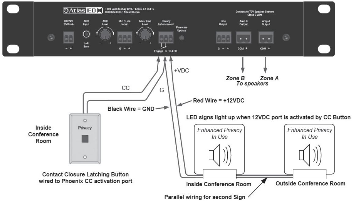
Wired Privacy Signs for Conference Room with ASP-MG2240 Application Example
