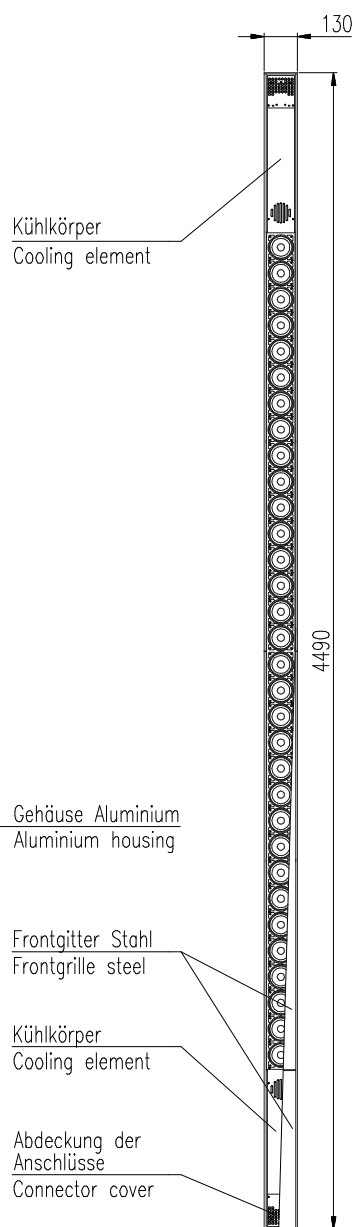
Front view
