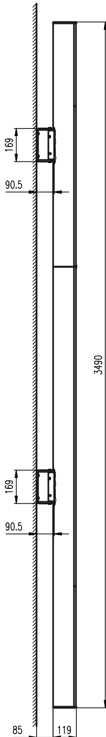
Side view
