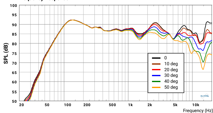
Frequency Response
