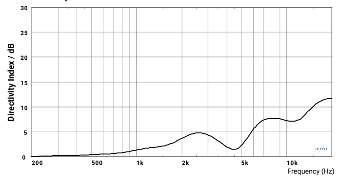
Directivity Index
